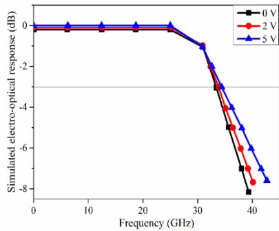
Fig. 7: Frequency response of a 120 \mu\text{m} phase shifter modulator under different DC biases.
