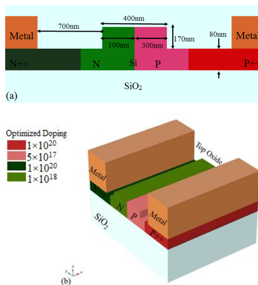
Fig. 1: (a) Schematic cross section of the lateral PN junction based optical phase shifter. (b) 3-D view of the phase shifter.
