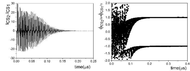
Figure 2: (Left) Intensity difference and (Right) phase difference of the two interacting SPLCSs for r = 1.7 and the initial distance of 48\mu\text{m} .
