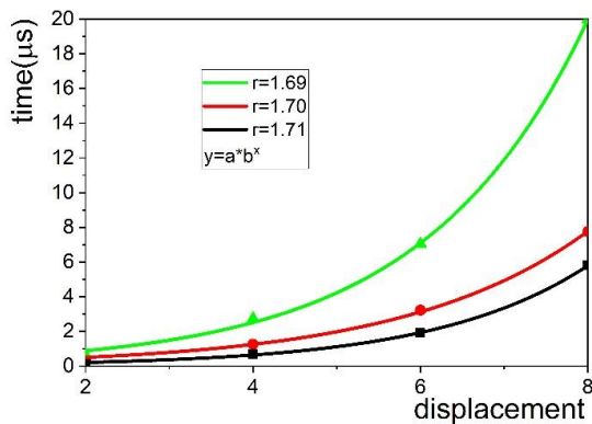
Figure 5: The time needed for the SPLCSs to move away from each other in the amount shown on horizontal axis for different values of the bifurcation parameter r . Their initial spacing is 48\mu m .
