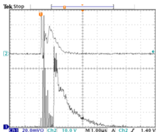
شکل (۴) (\text{He}=7, \text{N}_2=1, \text{CO}_2=2.2)^{\text{lit/min}}, V_{\text{D.C}}=20^{\text{kv}}
