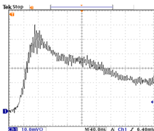
شکل (۷) (\text{He}=7, \text{N}_2=1.2, \text{CO}_2=2.2)^{\text{lit/min}}, V_{\text{D.C}}=17.5^{\text{kv}}
