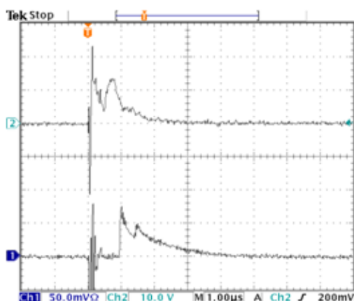
شکل (۶) (\text{He}=7, \text{N}_2=1.2, \text{CO}_2=2.2)^{\text{lit/min}}, V_{\text{D.C}}=17.5^{\text{kv}}
