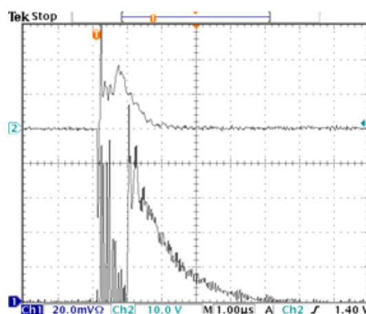
شکل (۳) (\text{He}=7, \text{N}_2=1.2, \text{CO}_2=2.4)^{\text{lit/min}}, V_{\text{D.C}}=20^{\text{kv}}
