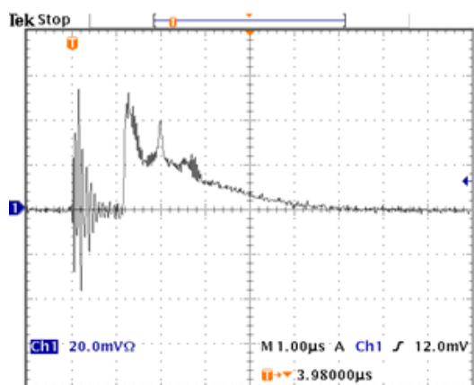
شکل (۵) (\text{He}=7, \text{N}_2=1.2, \text{CO}_2=2.2)^{\text{lit/min}}, V_{\text{D.C}}=15^{\text{kv}}
