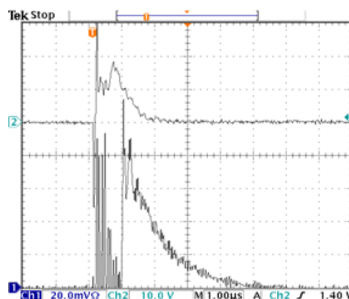
شکل (۲) (\text{He}=7, \text{N}_2=1.2, \text{CO}_2=2.2)^{\text{lit/min}}, V_{\text{D.C}}=20^{\text{kv}}
