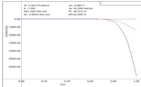
Fig. 3. I-V characteristics of CdS/CdTe solar cells without buffer layer
