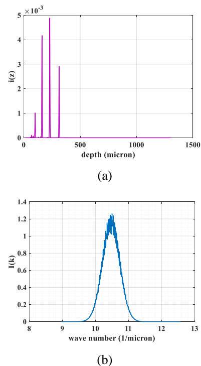
Fig. 1: A sample generated data, (a) z-space output (b) k-space output
