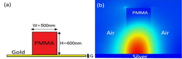
Figure 3: (a) Schematic representation of the SPPs from proposed waveguide (b) Mode distribution of optimal configuration.
