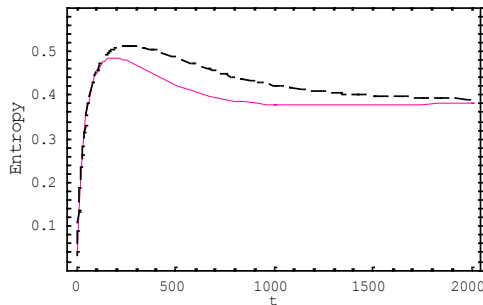
۳) کاهش آنتروپی \Omega_1 = .001 \Omega_2 = .0003 \gamma = .001 n = 3
