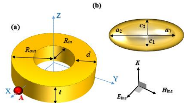
Figure 1: (a) The schematic representation of the gold NR. The point A is the near-field monitor point. (b) A simplified oblate spheroidal NS ( b_1 = a_1 , and b_2 = a_2 are the major axes).
