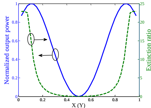
Figure 3: Normalized output power and extinction ratio from switched port 3 versus unequal power splitting coefficients
