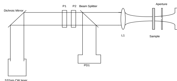
Figure 2 : experimental setup of closed aperture Z-scan
