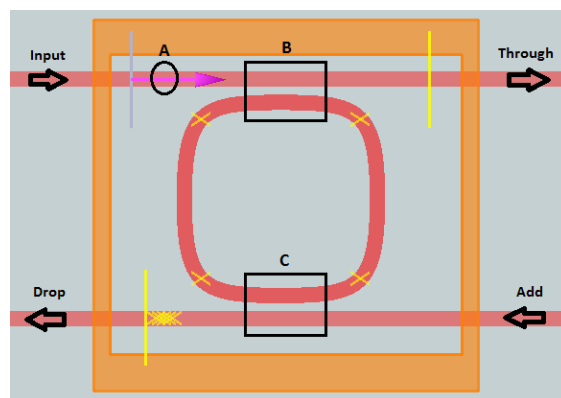
Fig. 1: Bezier micro ring resonator
